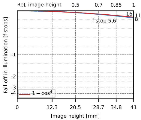
Fall-off in illumination Mag. 1x
