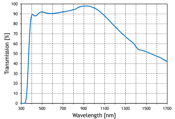
Transmission - inspec.x L 5.6/105 VIS/NIR 1x
