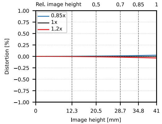
Distortion Mag. 0.85x ... 1.2x
